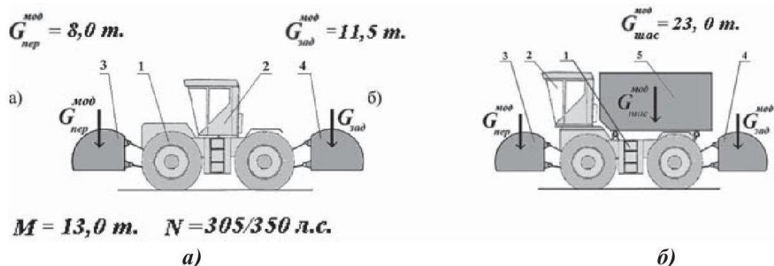
Fig. 2. Aggregation with the manufactured UEV (Claas company) technological and assembly adapters: a, b - MEV models Xerion Trac, Xerion Saddle Trac; 1 - MEV; 2 - control cabin, 3 and 4 - front and rear systems with adapters; Transport and Technology Adapter on Chassis 5
